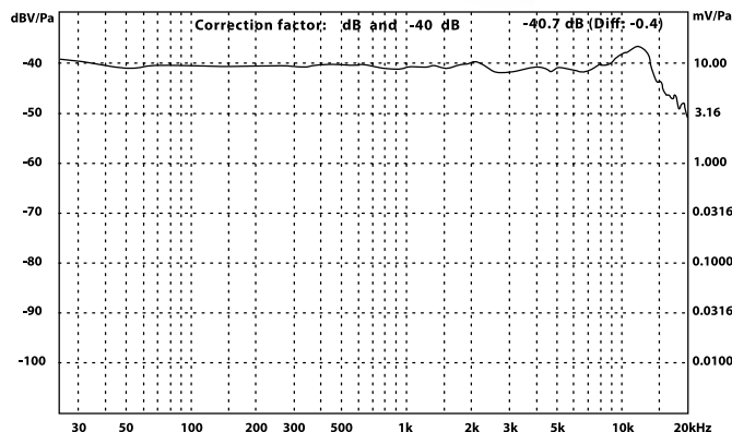
Microphone Frequency Response
