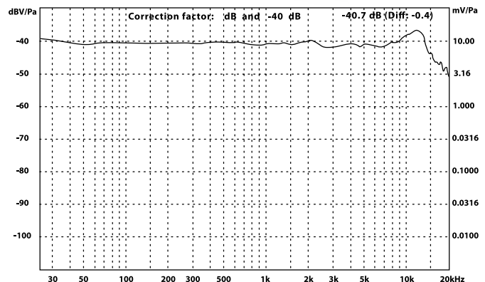
Microphone Frequency Response
