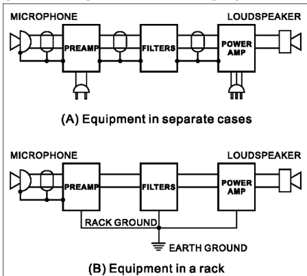
Figure 8 Examples of connections of shields to chassis
